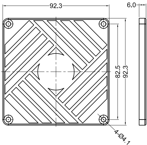
Finger Guard
