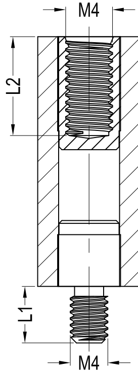
I/S Fig.2
