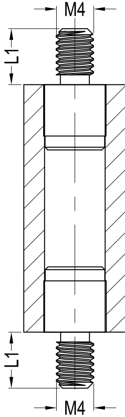
S/S Fig.1
