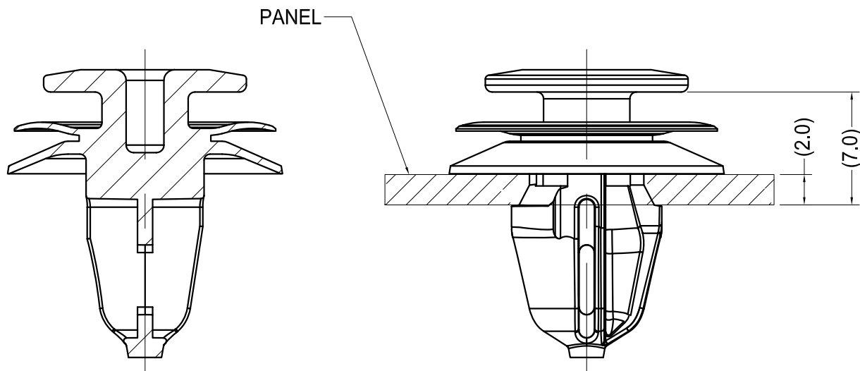
ASSEMBLY DETAILS
